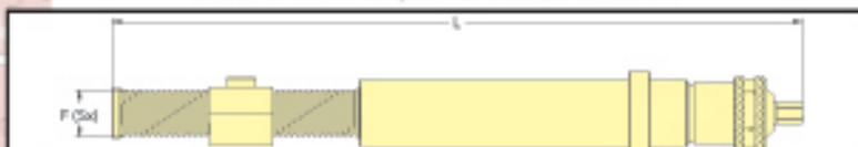
COPERCHIO GUIDA VITE/SCREW GUIDE COVER ED03
